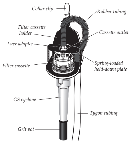
Figure 2. GS-1 Cyclone/cassette assembly in holder (Cat. No. 225-1)
